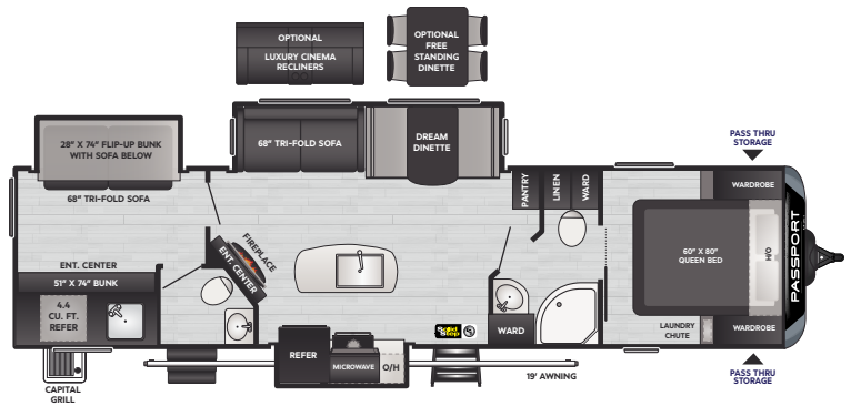
3300BK | WEIGHT 7995 | LENGTH 31' 11"
