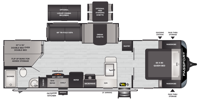
2900BH/WE | WEIGHT 6380 | LENGTH 33' 6"
