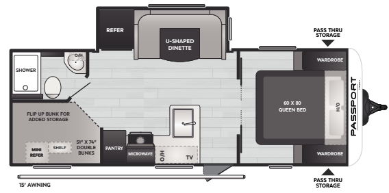
229BH/WE | WEIGHT 5590 | LENGTH 27' 4"
