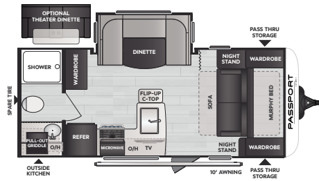
189RB/WE | WEIGHT 4883 | LENGTH 23' 1"
