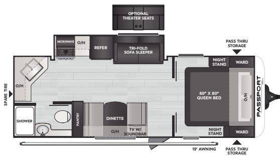
229RK/WE | WEIGHT 5590 | LENGTH 27' 4"
