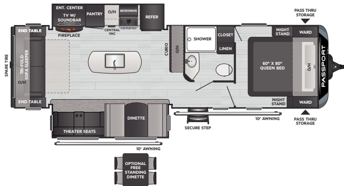
2870RL/WE | WEIGHT 7110 | LENGTH 33' 0"
