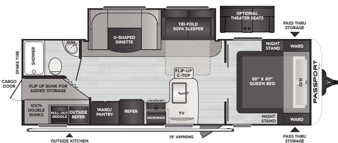
268BH/WE | WEIGHT 6170 | LENGTH 30' 4"
