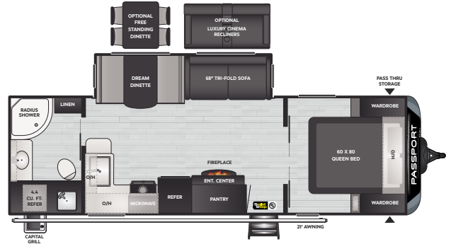
2605RB/WE | WEIGHT 6226 | LENGTH 30' 6"
