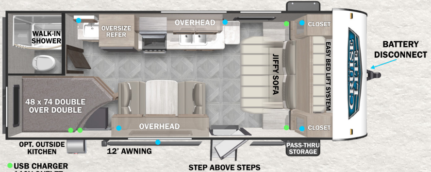
● USB CHARGER ● 110V OUTLET MODEL #: 19DBXL HITCH: 520 LBS UVW: 4,483 LBS LENGTH: 24'8"
