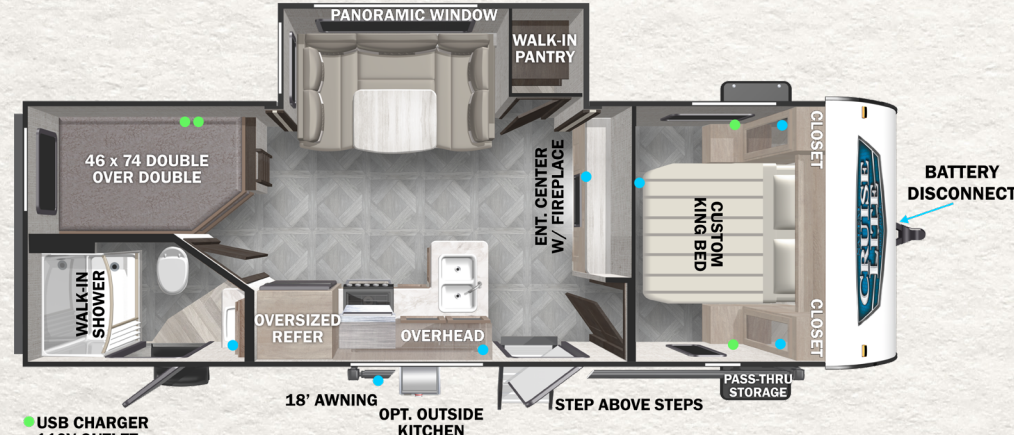
● USB CHARGER ● 110V OUTLET MODEL #: 240BHXL HITCH: 570 LBS UVW: 5,343 LBS LENGTH: 28'10"
