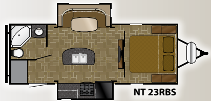
Length: 26' 11" Dry: 5,310 GVWR: 6,900 Height: 11' 2" Hitch: 625
