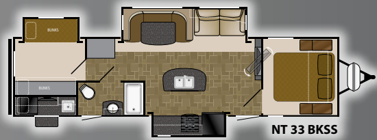
Length: 36' 10" Dry: 7,595 GVWR: 9,600 Height: 11' 4" Hitch: 695
