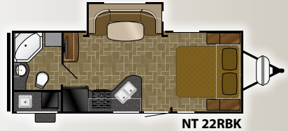
Length: 26' 4" Dry: 4,774 GVWR: 6,900 Height: 11' 2" Hitch: 440
