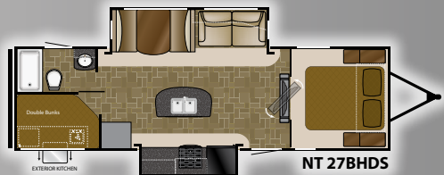
Length: 32' 8" Dry: 6,674 GVWR: 8,600 Height: 11' 4" Hitch: 780
