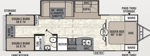
292 BHDS ♦ Exterior Length 33' 5"
