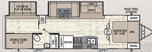
310 BHDS ♦ Exterior Length 35' 7"
