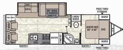
281 RLDLSLE ♦ Exterior Length 31' 8"
