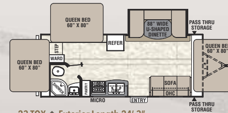
23 TOX ♦ Exterior Length 24' 3"
