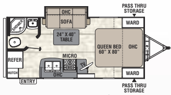
192 RBS ♦ Exterior Length 22' 6"
