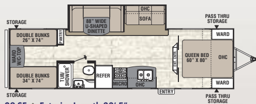
29 SE ♦ Exterior Length 33' 5"
