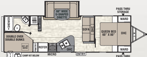
275 BHS ♦ Exterior Length 31' 8"
