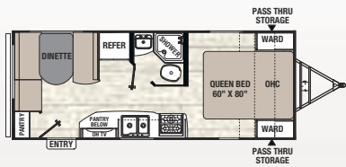
204 RD ♦ Exterior Length 24' 7"
