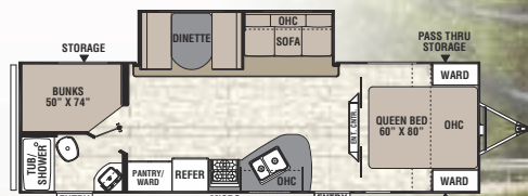
28 SE ♦ Exterior Length 31' 11"
