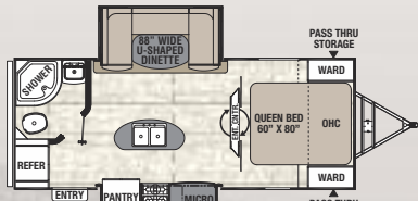
233 RBS ♦ Exterior Length 24' 11"
