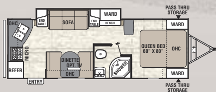
246 RKS ♦ Exterior Length 28' 3"
