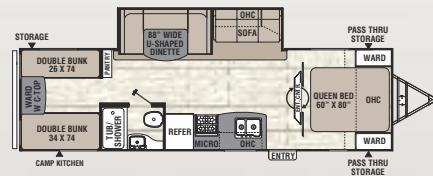
292 BHDLSLE ♦ Exterior Length 33' 5"
