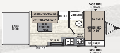
17BL SE ♦ Exterior Length 20' 4"
