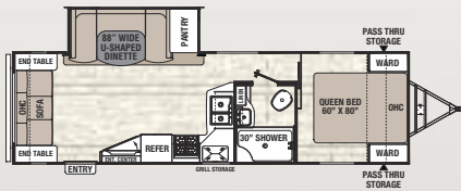
279 RLDLSLE ♦ Exterior Length 31' 11"
