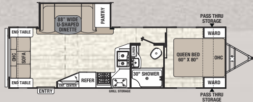
279 RLDS ♦ Exterior Length 31' 11"
