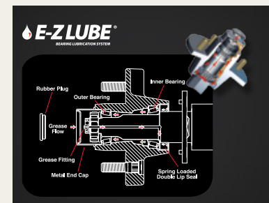
E-Z lube axles allow you to lubricate your wheel bearings quickly and easily without disassembly
