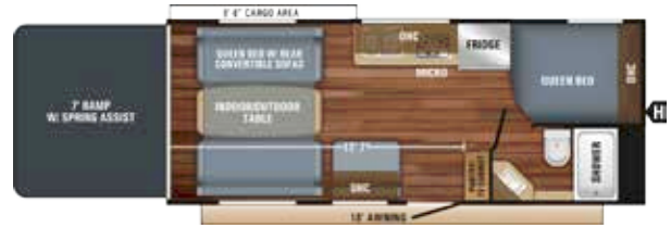
OCTANE SUPER LITE | 222 Ext. Lgth: 26' 5" Ext. Ht: 135" Unloaded Wt. (lbs): 5,445 Sleeps: 6
