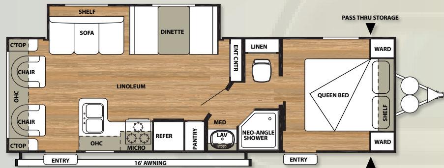
252RL DRY SHIP WEIGHT: 5352
