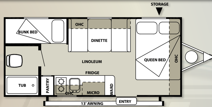
195BH DRY SHIP WEIGHT: 3003
