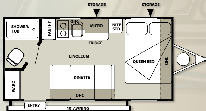
185RB DRY SHIP WEIGHT: 2881
