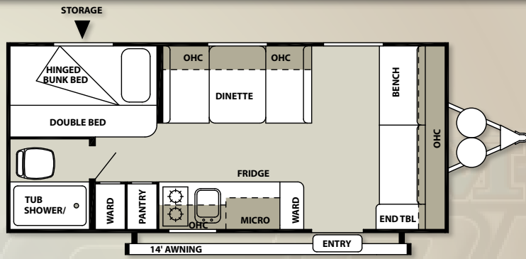
174BH DRY SHIP WEIGHT: 3252
