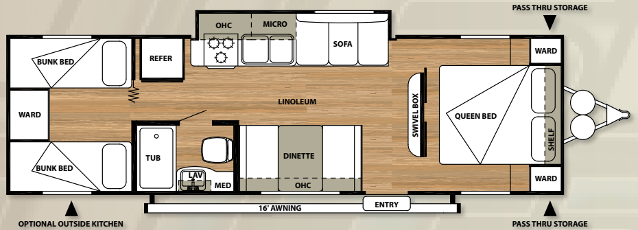
281QB DRY SHIP WEIGHT: 5438
