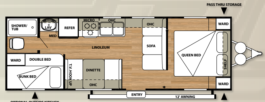
261BH DRY SHIP WEIGHT: 4313
