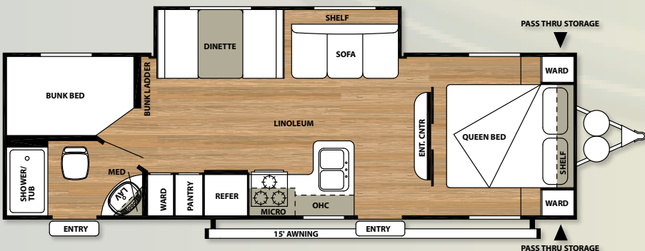
262BH DRY SHIP WEIGHT: 5801
